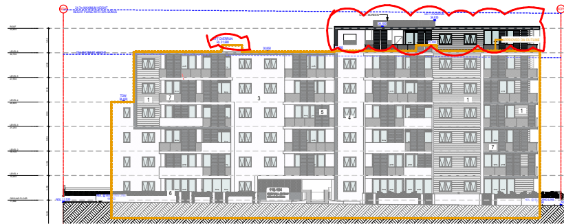
WEST ELEVATION (RESTWELL ST)
