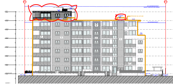
SOUTH ELEVATION ( MACAULEY AVE)
